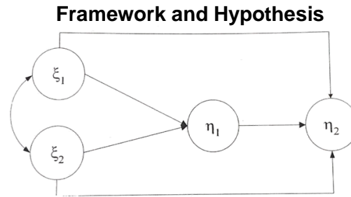
Figure 2. Relationship Flow Framework between Latent Variables
