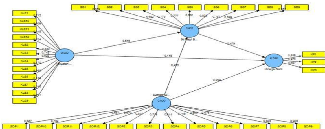
Figure 1. Coefficient
